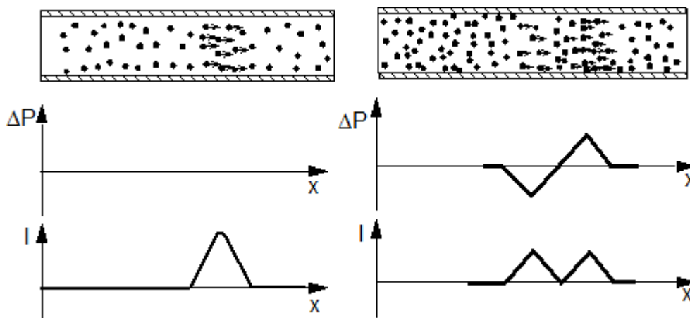
Fig.: 1.2.8. Displacement of a small zone with drifting particles left: Starting position right: Situation after a few time steps
