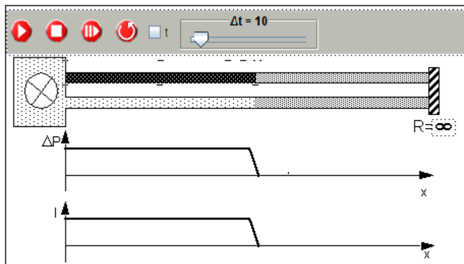
Fig.: 1.4.8. Simulation of a current moving towards the closed end of a double line with R = \infty
