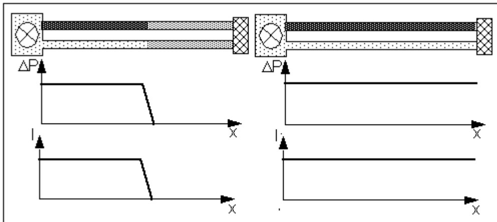
Fig.: 1.4.11. Left: Front of a current moving towards the reflection free ending of a double line Right: State of pressure and current after "reflection"
