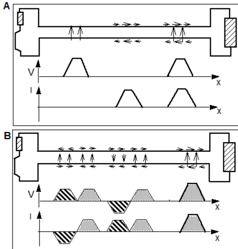
Fig.: 1.2.9. Displacement of a pulse and its components on a double line
