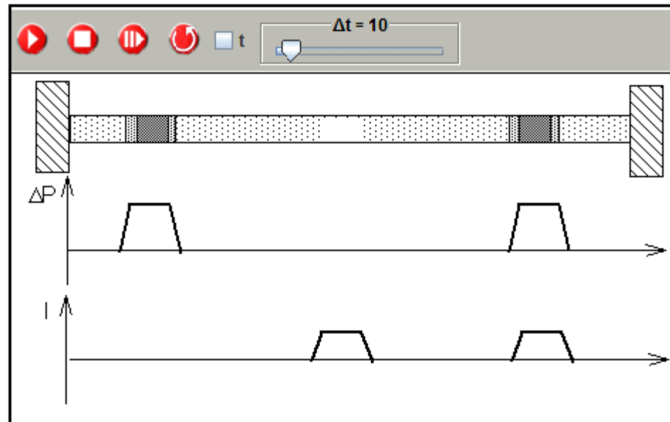
Fig.: 1.2.14. Simulation of the displacement of a pulse with a changed ratio of \Delta P/I . By using different starting situation for \Delta P and I it can be checked whether the rule, stated above, is generally valid.
