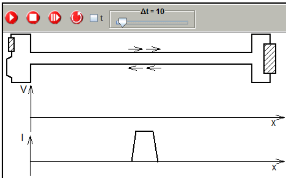
Fig.: 1.2.7. Simulation of a zone with drifting free electrons on a double line It is advised to activate the simulation by using the step button.
