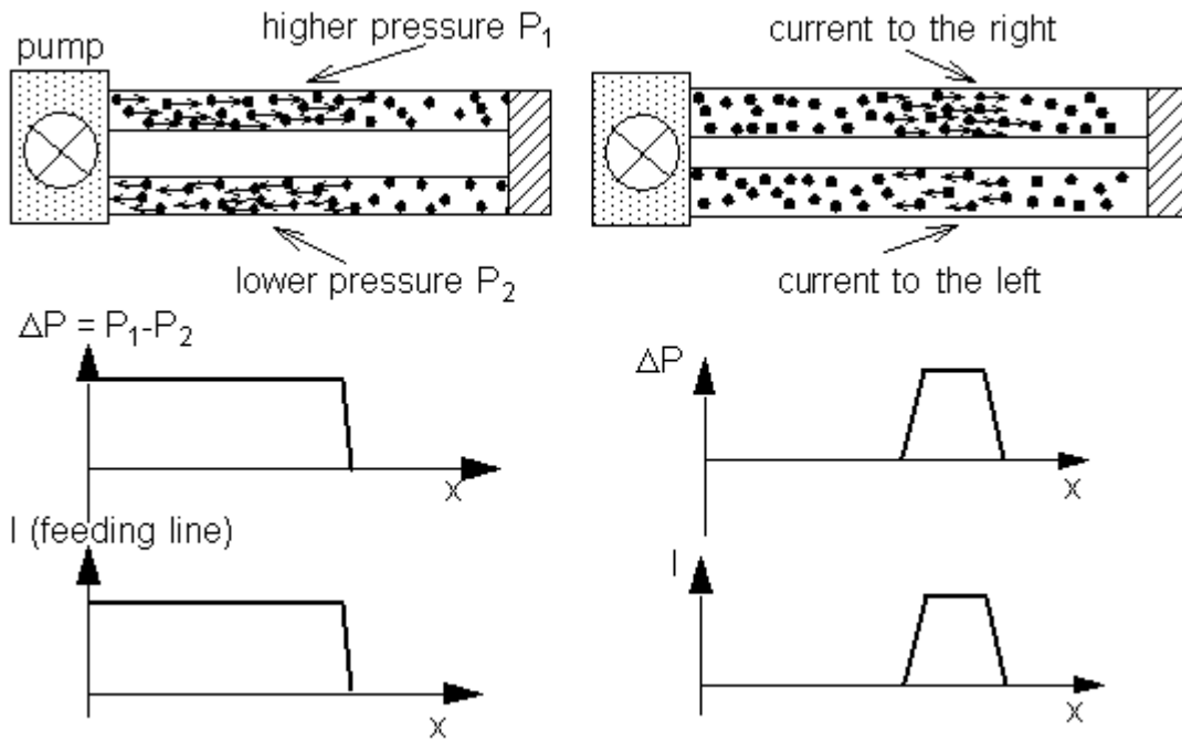
Fig.: 1.4.2. Pressure difference and current for a starting flow (left) and a pulse (right) on a double line
