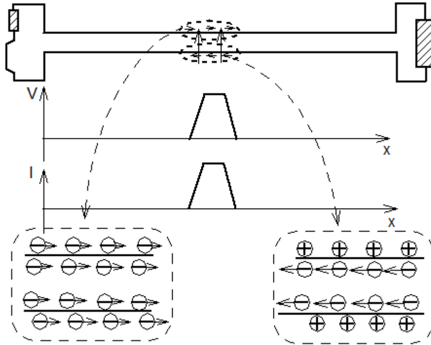
Fig.: 1.2.8. Microscopic view of a pulse on a double line
