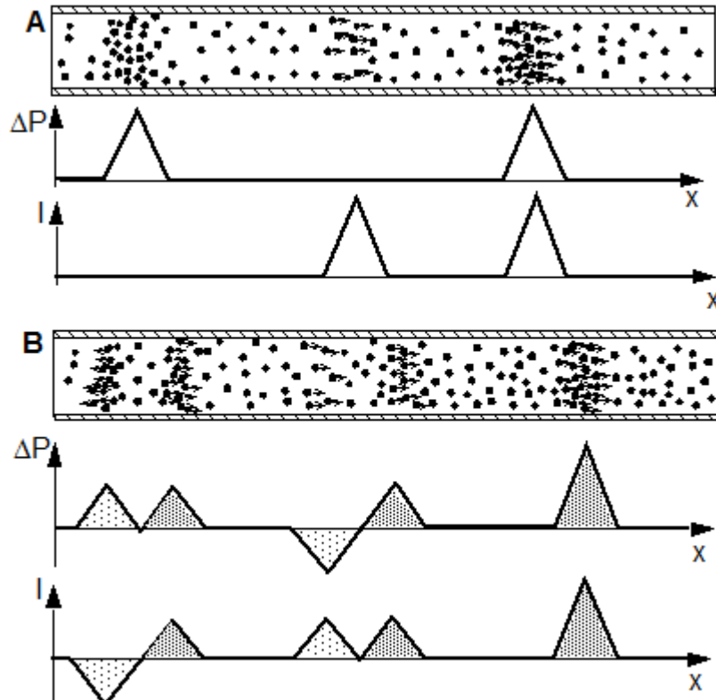
Fig.: 1.2.10. A: Starting situation: A pulse and its components at different locations
