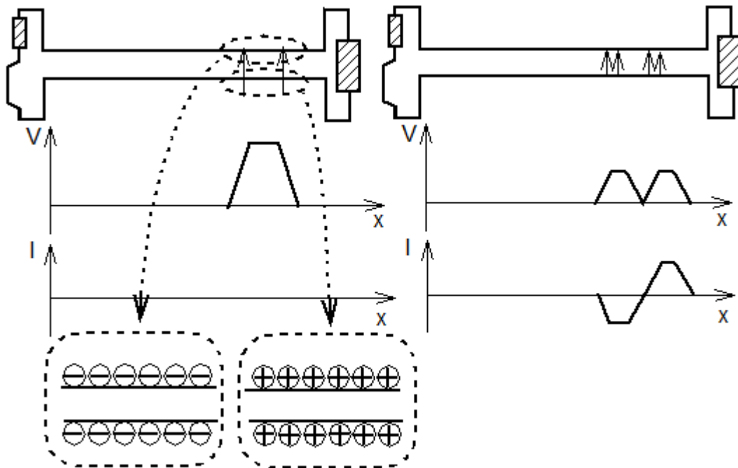
Fig.: 1.2.4. Displacement of a zone with surface charges on a double line Left: Starting position; Right: Displacement after a few time steps
