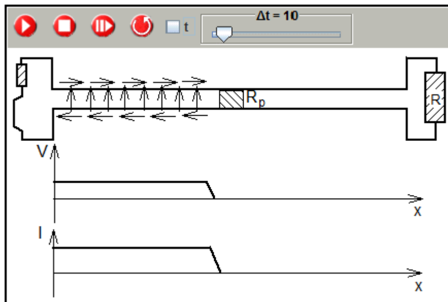
Fig.: 2.5.3. Double line with an additional resistor in parallel with the terminating resistor
