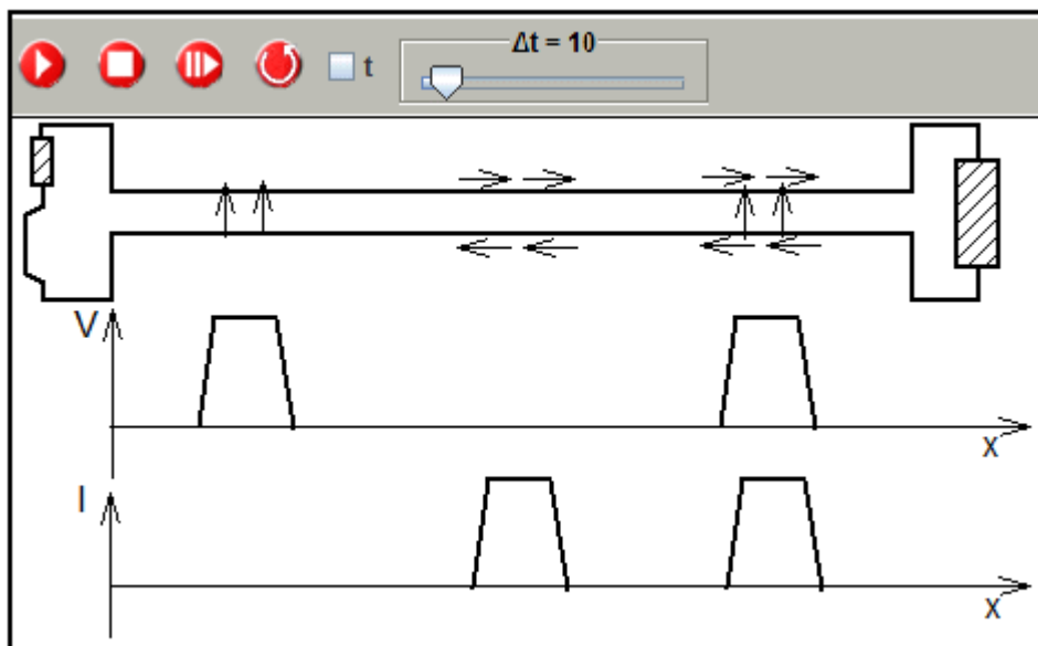
Fig.: 1.2.10. Simulation of the transmission of a pulse and its components on a double line
