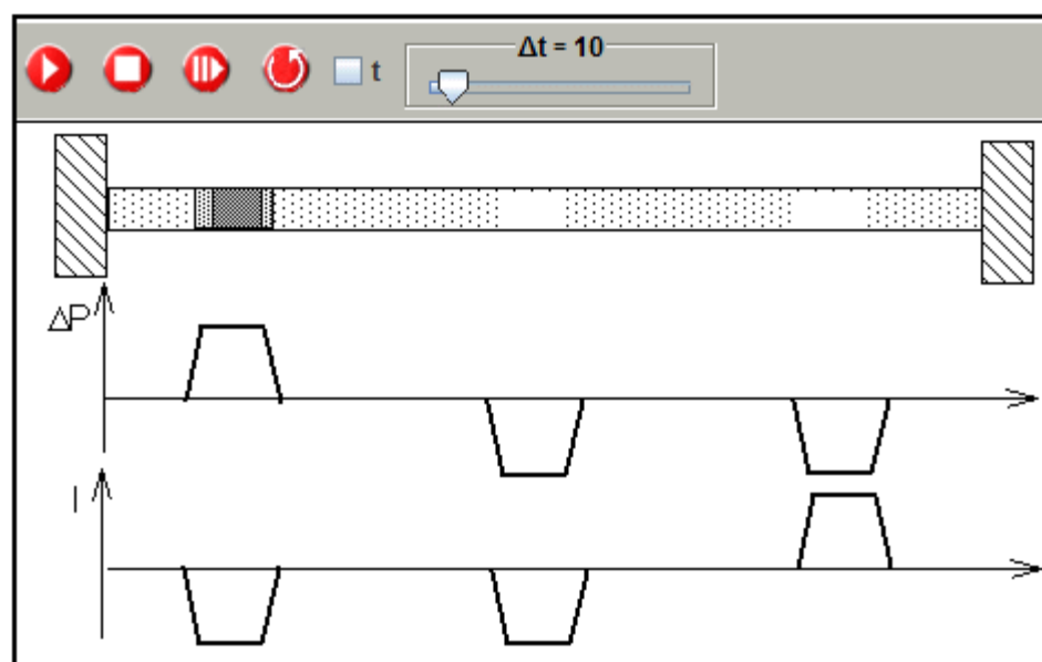
Fig.: 1.2.12. Simulation of pulse transmission in opposite directions
