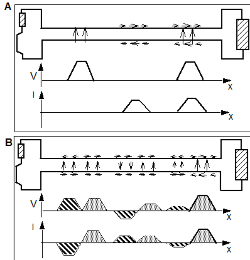
Fig.: 1.2.11. Displacement of a pulse and its components with arbitrary ratio of V/I A: Starting position; B: Situation after a few time steps
