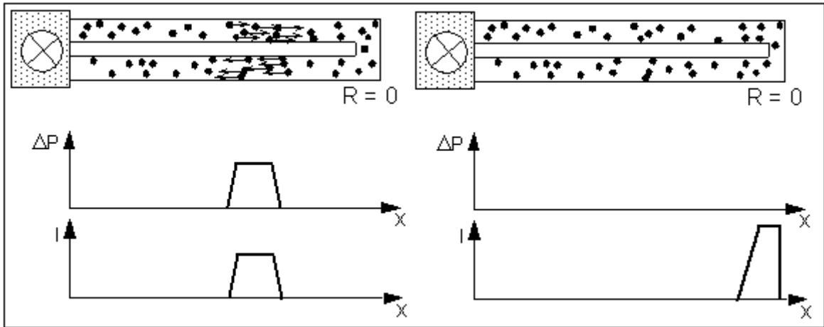
Fig.: 1.4.9. Left: A pulse moving towards the shorted ends of a double line Right: Moment of reflection
