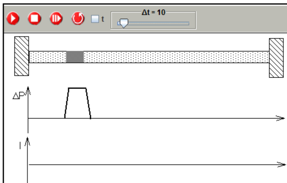
Fig.: 1.2.7. Simulation of the displacement of a small pressure zone
