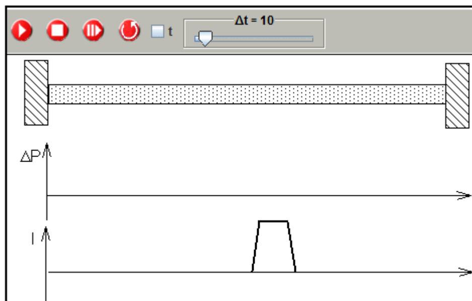
Fig.: 1.2.9. Simulation of the propagation of a zone with drifting particles but no change in pressure
