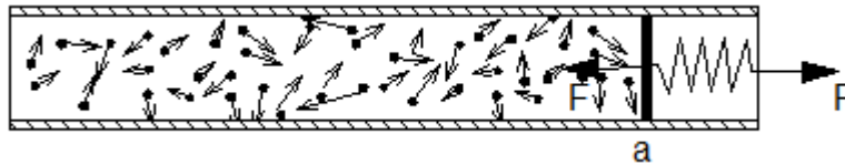
Fig.: 1.1.2. Pressure on a wall, caused by colliding particles
