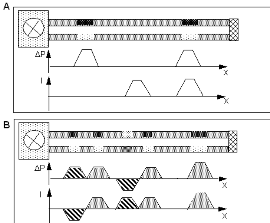
Fig.: 1.4.3. A: Starting situation: 2 separated components and a complete pulse
