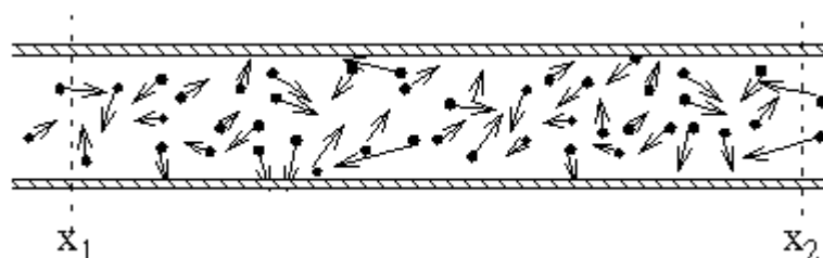
Fig.: 1.1.1. Thermal velocity of gas atoms or molecules
