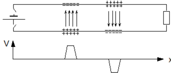
Fig.: 1.2.2. Two voltage pulses of opposite polarity on a double line
