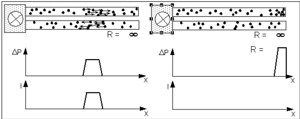
Fig.: 1.4.5. Left: A pulse moving towards a closed end of a double line Right: Moment of reflection
