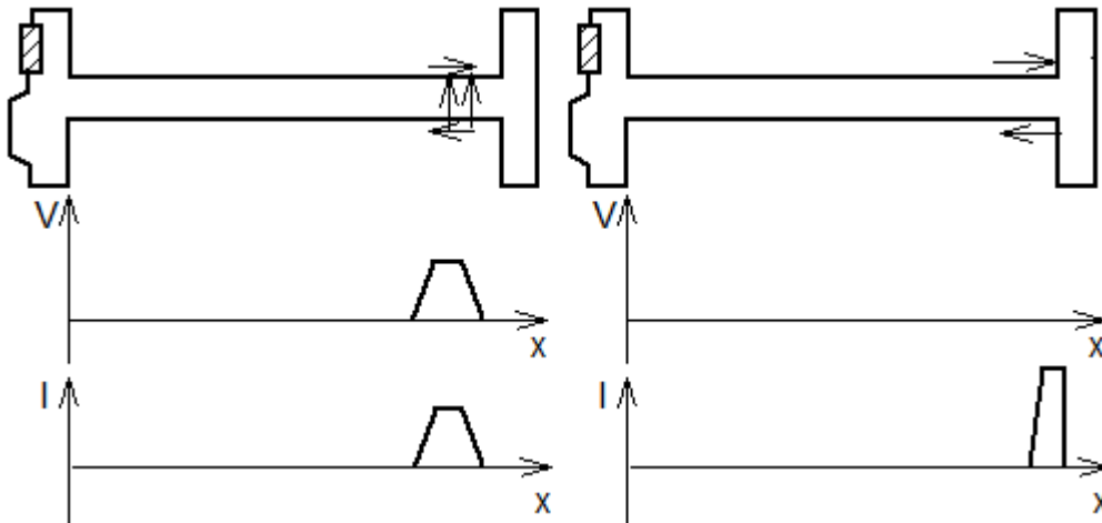
Fig.: 2.3.2. Left: A pulse moving towards the shorted ends of a double line ( R=0 \Omega ) Right: Moment of reflection
