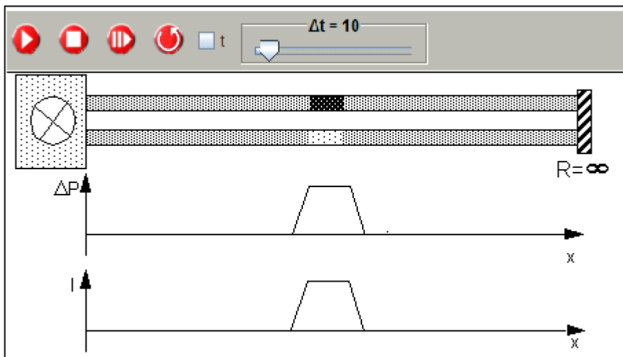
Fig.: 1.4.6. Simulation of a pulse reflection at a closed end of a double line ( R = \infty )
