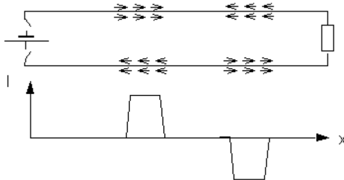
Fig.: 1.2.3. Zones with drifting electrons on a double line
