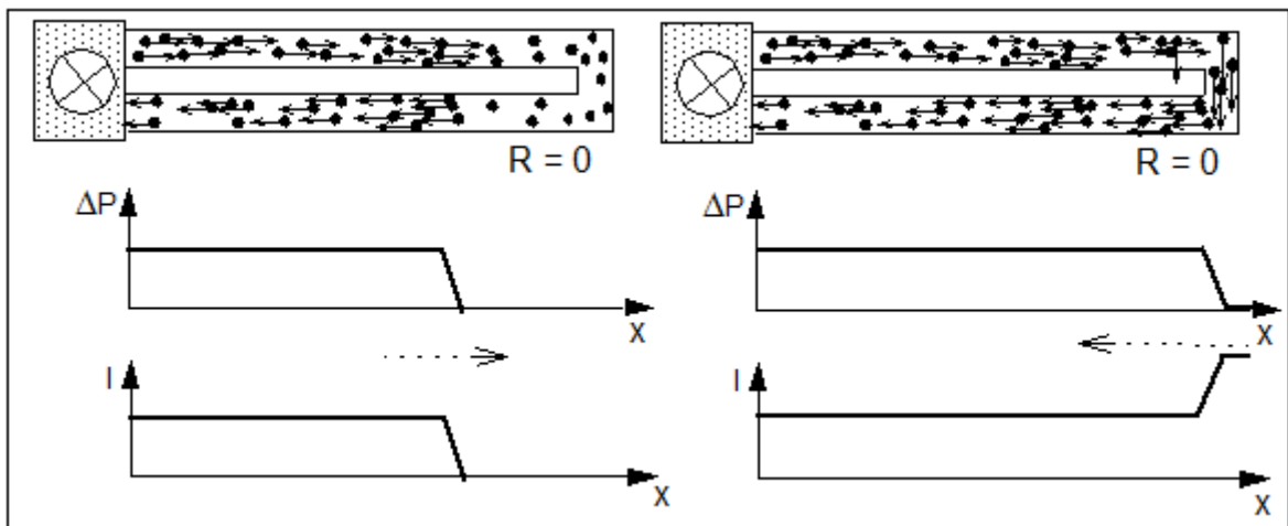
Fig.: 1.4.10. Left: The front of a current moving towards the shorted ends of a double line Right: State of pressure and current at the moment of reflection
