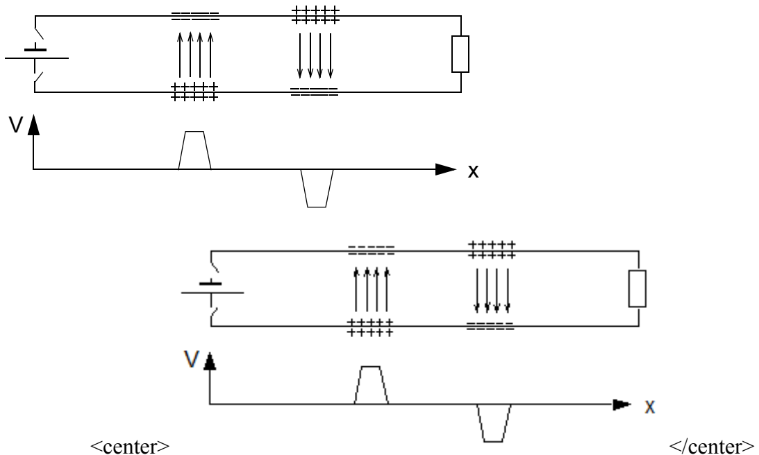
Fig.: 2.4.1. Voltage pulses and surface charges on a double line
