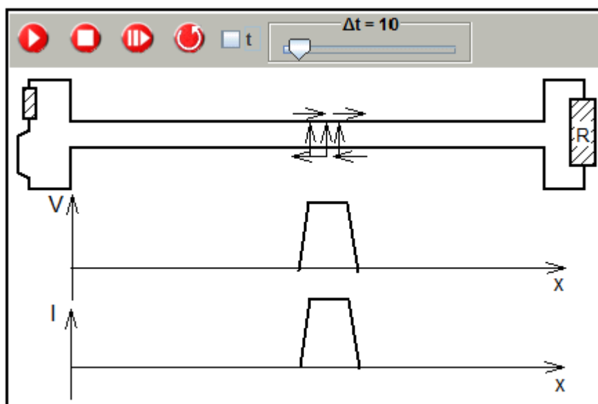
Fig.: 2.3.3. Simulation of a pulse transmission and reflection on a double line with various terminating resistors
