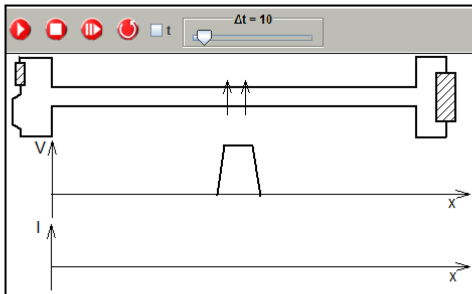
Fig.: 1.2.5. Simulation of voltage zone on a double line
