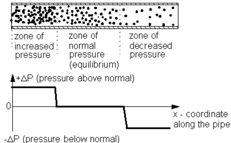
Fig.: 1.2.1. Graphical representation of pressure along a pipe
