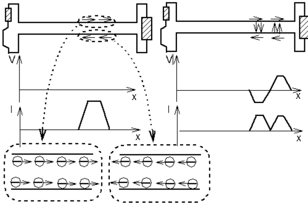
Fig.: 1.2.6. Displacement of a zone with drifting free electrons on a double line Left: Starting position; Right: Displacement after a few time steps
