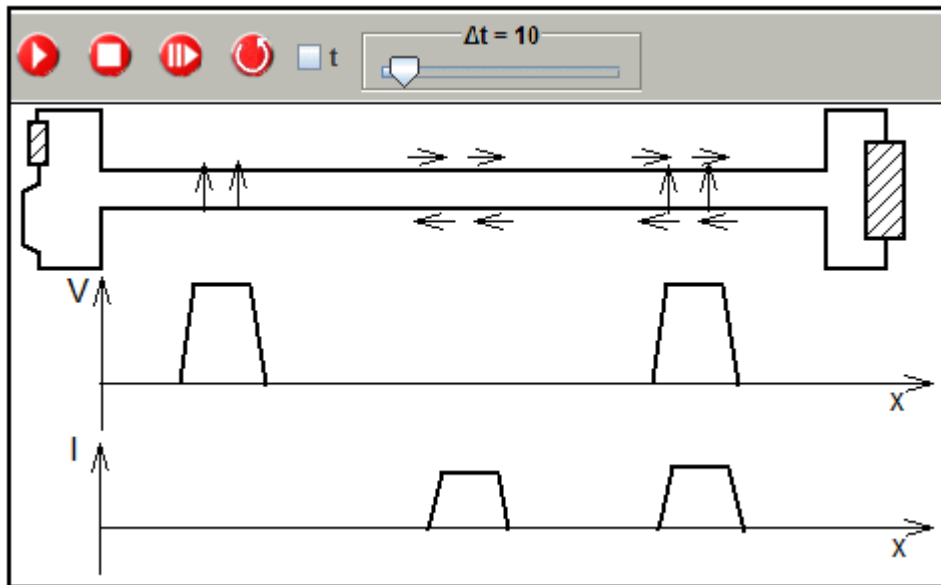
Fig.: 1.2.12. Simulation of a pulse and its components with arbitrary ratio of V/I
