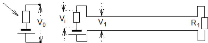
Fig.: 2.5.1. Double line with voltage source and internal resistor
