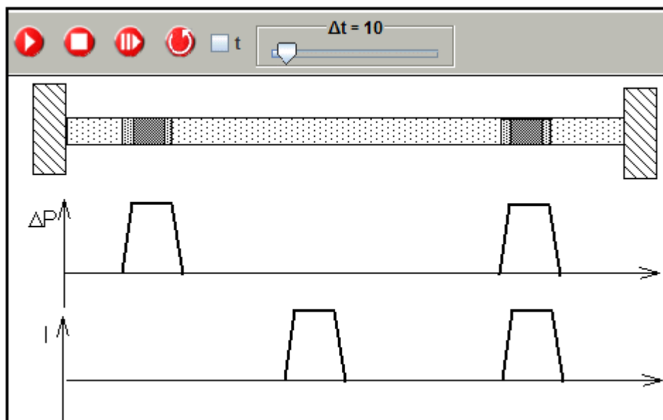
Fig.: 1.2.11. Simulation of the displacement of a pulse and its two components
