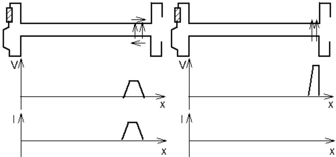
Fig.: 2.3.1. Left: A pulse moving towards the open ends of a double line ( R = \infty \Omega ) Right: Moment of reflection
