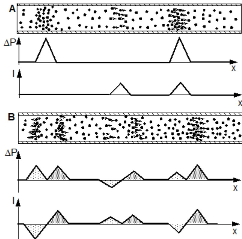
Fig.: 1.2.13. Displacement of a pulse with a changed ratio of \Delta P/I
