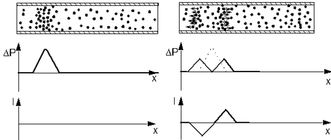
Fig.: 1.2.6. Displacement of a small zone with increased pressure left: Starting position right: Position after a few time steps
